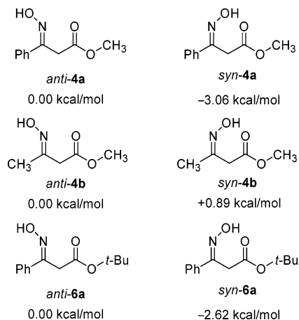
FIGURE 1. Calculated relative energy for 4a , 4b , and 6a (syn/anti against ester moiety).
