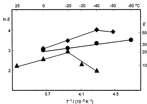
FIGURE 2. Temperature effect in the lipase-catalyzed resolution of ( \pm )-2: \blacklozenge , in acetone; \bullet , in THF; \blacktriangle , in Et 2 O.
