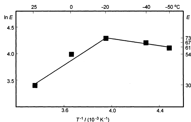
FIGURE 3. Temperature effect in the lipase-catalyzed resolution of ( \pm )-3 in acetone.
